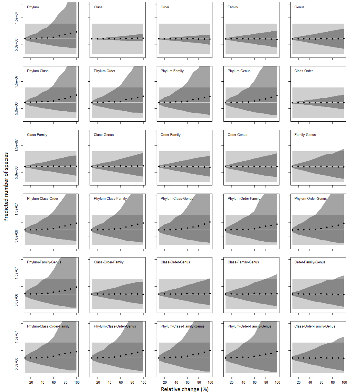
Figure S2. Sensitivity analysis due to changes in higher taxonomy. One potential caveat in our approach is the degree to which estimations of the number of species may change if higher taxonomy changes. To test this effect we performed a sensitivity analysis in which the number of species was calculated after altering the number of higher taxa. We used Animalia as a test case. For each possible combination of taxonomic levels, we added or removed a random proportion of taxa from 10 to 100% of the current number of taxa and recalculated the number of species using the method described in this paper. The approach was repeated 1000 times and the average and 95% confidence limits of the simulations are shown as points and dark areas, respectively. Light gray lines and boxes indicate the currently estimated number of species and its 95% prediction interval, respectively. Our current estimation of the number of species appear remarkably robust to changes in higher taxonomy. As noted, results were only sensitive to changes in the number of phyla, and only when this number changed by over 50% relative to the number of currently described phyla. For all other taxonomic levels, expected changes led to predictions that remain within the confidence intervals of the currently estimated number of species.
