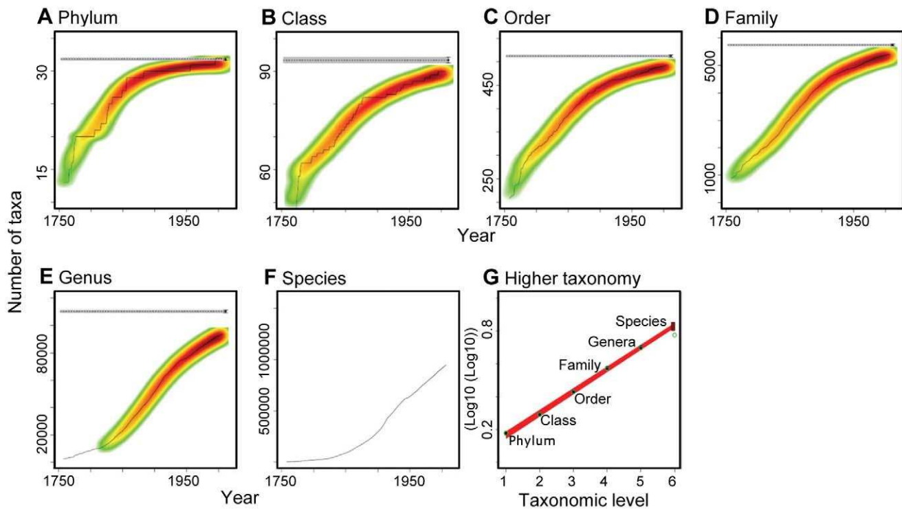
Figure 1. Predicting the global number of species in Animalia from their higher taxonomy. (A–F) The temporal accumulation of taxa (black lines) and the frequency of the multimodel fits to all starting years selected (graded colors). The horizontal dashed lines indicate the consensus asymptotic number of taxa, and the horizontal grey area its consensus standard error. (G) Relationship between the consensus asymptotic number of taxa and the numerical hierarchy of each taxonomic rank. Black circles represent the consensus asymptotes, green circles the catalogued number of taxa, and the box at the species level indicates the 95% confidence interval around the predicted number of species (see Materials and Methods).
